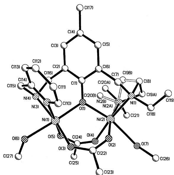
Fig. 5 An ORTEP drawing of the molecular structure of 5 showing the atom labelling; thermal ellipsoids for the non-hydrogen atoms are drawn at the 50% probability level. Selected bond lengths and angles at the metal atoms: Ni(1)–O(1), 2.023(3); Ni(1)–N(3), 2.066(4); Ni(1)–O(3), 2.06(4); Ni(1)–O(5), 2.070(4); Ni(1)–N(4), 2.092(5); Ni(1)–O(6), 2.142(4); Ni(2)–O(2), 2.004(5); Ni(2)–O(1), 2.011(4); Ni(2)–O(4), 2.038(4); Ni(2)–N(1), 2.122(4); Ni(2)–N(2A), 2.149(6); Ni(2)–N(2B), 2.152(7); Ni(2)–O(7), 2.379(6); Ni(1)–Ni(2), 3.4268(11) Å. Ni(1)–O(1)–Ni(2), 116.31(16); O(2)–C(22)–O(3), 126.1(5); O(4)–C(24)–O(5), 125.6(6); O(1)–Ni(1)–O(6), 175.50(15); N(3)–Ni(1)–O(5), 174.28(16); O(3)–Ni(1)–N(4), 169.53(17); O(4)–Ni(2)–N(1), 172.13(18); O(2)–Ni(2)–N(2A), 166.6(3); O(2)–Ni(2)–N(2B), 169.2(52); O(1)–Ni(1)–O(7), 166.20(16)°.
