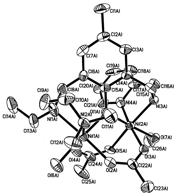
Fig. 4 An ORTEP drawing of the molecular structure of 4 showing the atom labelling; thermal ellipsoids for the non-hydrogen atoms are drawn at the 50% probability level. Selected bond lengths and angles at the metal atoms: Ni(1A)–O(1A), 1.992(4); Ni(1A)–O(4A), 2.051(5); Ni(1A)–O(2A), 2.065(5); Ni(1A)–N(1A), 2.161(6); Ni(1A)–O(6A), 2.171(5); Ni(1A)–N(2A), 2.175(6); Ni(2A)–O(5A), 2.014(5); Ni(2A)–O(1A), 2.023(5); Ni(2A)–N(4A), 2.027(6); Ni(2A)–N(3A), 2.058(5); Ni(2A)–O(3A), 2.074(5); Ni(2A)–O(7A), 2.145(4); Ni(1A)–Ni(2A), 3.4171(14) Å. Ni(1A)–O(1A)–Ni(2A), 116.7(2); O(4A)–C(24A)–O(5A), 117.9(7); O(2A)–C(22A)–O(3A), 127.1(7); O(2A)–Ni(1A)–N(1A), 173.5(2); O(1A)–Ni(1A)–O(6A), 171.63(19); O(4A)–Ni(1A)–N(2A), 167.4(2); O(1A)–Ni(2A)–O(7A), 175.39(18); O(3A)–Ni(2A)–N(4A), 174.0(2); N(3A)–Ni(2A)–O(5A), 169.7(2)°.
