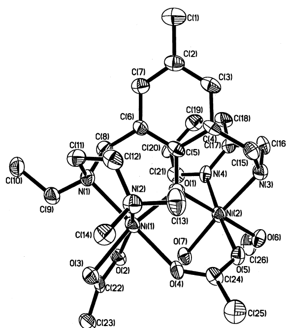
Fig. 2 An ORTEP drawing of the molecular structure of 2 showing the atom labelling; thermal ellipsoids for the non-hydrogen atoms are drawn at the 50% probability level. Selected bond lengths and angles at the metal atoms: Ni(1)–O(1), 2.019(4); Ni(1)–O(4), 2.065(4); Ni(1)–N(2), 2.082(5); Ni(1)–O(2), 2.125(4); Ni(1)–N(1), 2.131(5); Ni(1)–O(3), 2.134(4); Ni(2)–O(1), 2.042(4); Ni(2)–N(4), 2.042(5); Ni(2)–O(5), 2.060(4); Ni(2)–O(7), 2.067(4); Ni(2)–N(3), 2.078(5); Ni(2)–O(6), 2.143(4); Ni(1)–Ni(2), 3.5419(12) Å. Ni(1)–O(1)–Ni(2), 121.40(19); O(4)–C(22)–O(5), 117.3(6); O(4)–Ni(1)–N(1), 177.32(18); N(2)–Ni(1)–O(2), 160.28(18); O(1)–Ni(1)–O(3), 159.52(16); O(1)–Ni(2)–O(6), 178.27(16); O(7)–Ni(2)–N(3), 169.74(18); N(4)–Ni(2)–O(5), 175.16(18)°.
