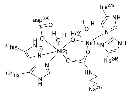
Fig. 1 Schematic depiction of the active site in urease.
