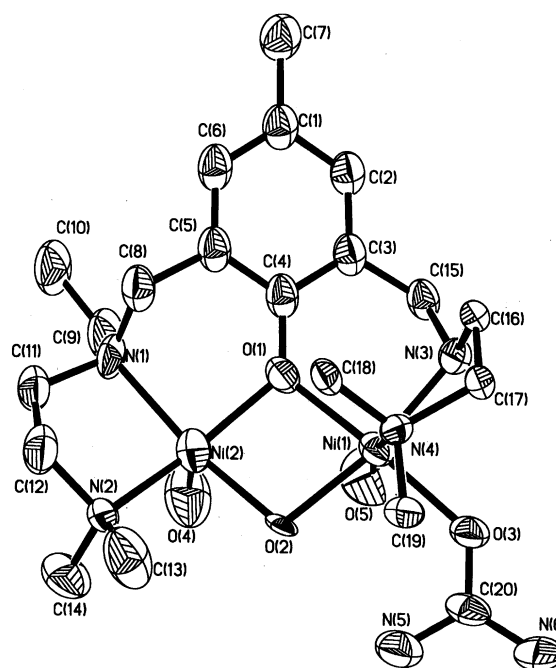
Fig. 6 An ORTEP drawing of the molecular structure of 6 showing the atom labelling; thermal ellipsoids for the non-hydrogen atoms are drawn at the 50% probability level. Selected bond lengths and angles at the metal atoms: Ni(1)–O(1), 2.016(5); Ni(1)–O(2), 2.032(4); Ni(1)–O(3), 2.038(6); Ni(1)–N(3), 2.054(6); Ni(1)–N(4), 2.110(6); Ni(1)–O(5), 2.153(7); Ni(2)–O(2), 1.940(5); Ni(2)–O(1), 1.960(5); Ni(2)–O(4), 2.041(7); Ni(2)–N(2), 2.069(7); Ni(2)–N(1), 2.091(7); Ni(1)–Ni(2), 3.0495(18) Å. Ni(1)–O(1)–Ni(2), 100.2(2); Ni(1)–O(2)–Ni(2), 100.3(2); N(4)–Ni(1)–O(5), 172.8(3); O(1)–Ni(1)–O(3), 171.7(2); N(3)–Ni(1)–O(2), 168.8(2); N(1)–Ni(2)–O(2), 167.1(2); N(2)–Ni(2)–O(1), 152.8(2); O(4)–Ni(2)–N(1), 100.3(3); O(4)–Ni(2)–O(2), 91.7(3); O(4)–Ni(2)–O(1), 104.1(3); O(4)–Ni(2)–N(2), 103.0(3)°.
