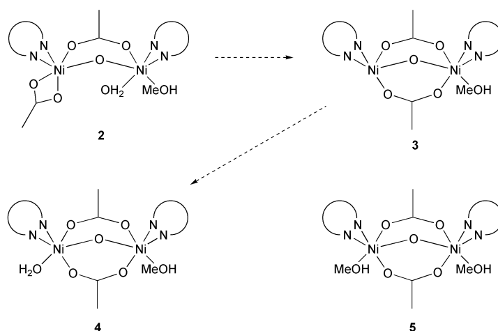
Scheme 1 Schematic representations of the dinickel(II) cores present in 2–5.
