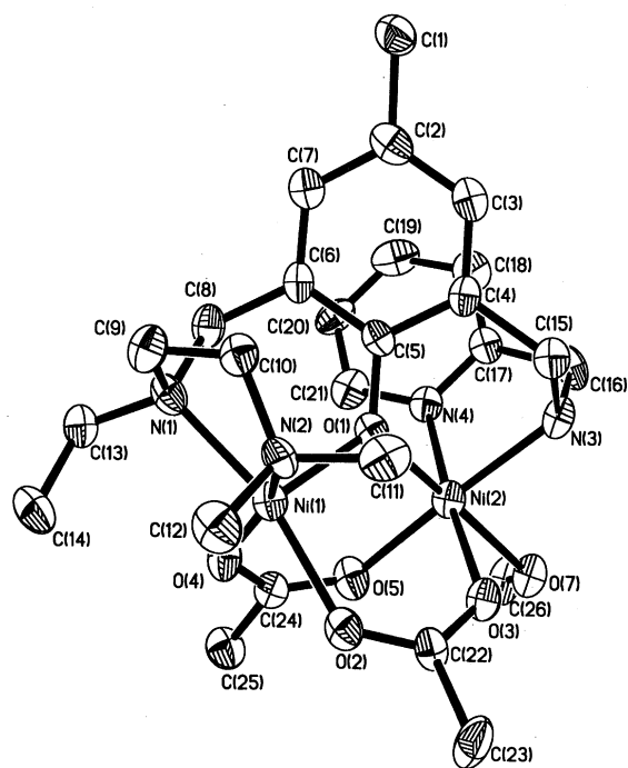
Fig. 3 An ORTEP drawing of the molecular structure of 3 showing the atom labelling; thermal ellipsoids for the non-hydrogen atoms are drawn at the 50% probability level. Selected bond lengths and angles at the metal atoms: Ni(1)–O(1), 1.948(4); Ni(1)–O(4), 1.983(4); Ni(1)–O(2), 2.058(5); Ni(1)–N(1), 2.089(6); Ni(1)–N(2), 2.103(5); Ni(2)–O(1), 2.001(4); Ni(2)–O(5), 2.039(5); Ni(2)–N(4), 2.067(6); Ni(2)–O(3), 2.079(4); Ni(2)–N(3), 2.083(5); Ni(2)–O(7), 2.128(4); Ni(1)–Ni(2), 3.3346(14) Å. Ni(1)–O(1)–Ni(2), 115.2(2); O(4)–C(24)–O(5), 126.9(6); O(2)–C(22)–O(3), 115.9(6); O(1)–Ni(2)–O(7), 175.20(17); N(4)–Ni(2)–O(3), 175.1(2); N(3)–Ni(2)–O(5), 170.81(19); N(1)–Ni(1)–O(2), 164.99(19); N(2)–Ni(1)–O(4), 160.5(2); O(1)–Ni(2)–N(1), 96.40(19); O(1)–Ni(1)–O(4), 99.74(18); O(1)–Ni(1)–O(2), 98.42(18); O(1)–Ni(1)–N(2), 99.57(19)°.
